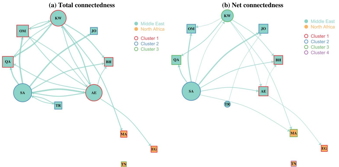
Figure 5. Connectedness from the standard VAR model
