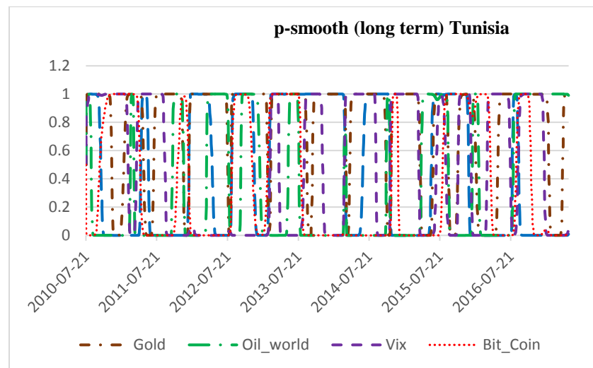
Fig. A2. Smoothing short and long-term correlations between the stock markets and global factors.
