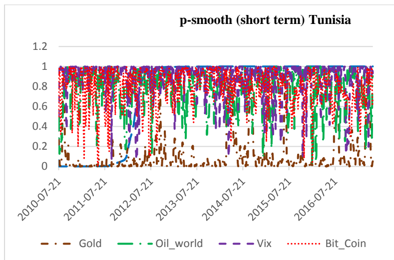
Fig. A2. Smoothing short and long-term correlations between the stock markets and global factors.
