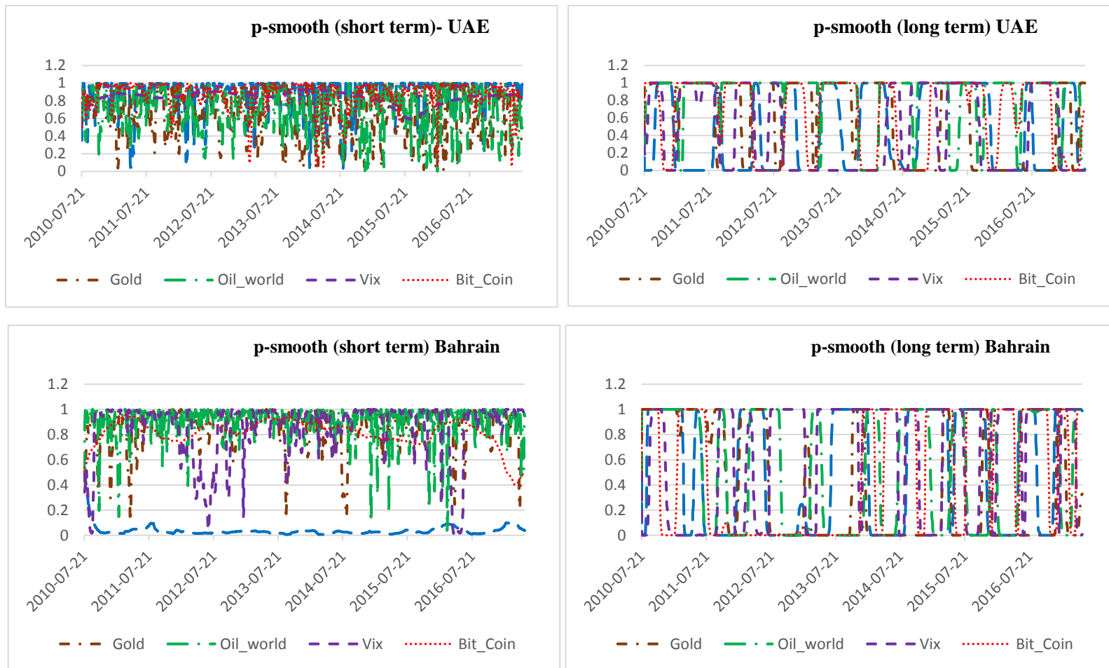
Fig. A1. Smoothing probability of the positive correlation regime between the stock and global factors in the short- and long term.
