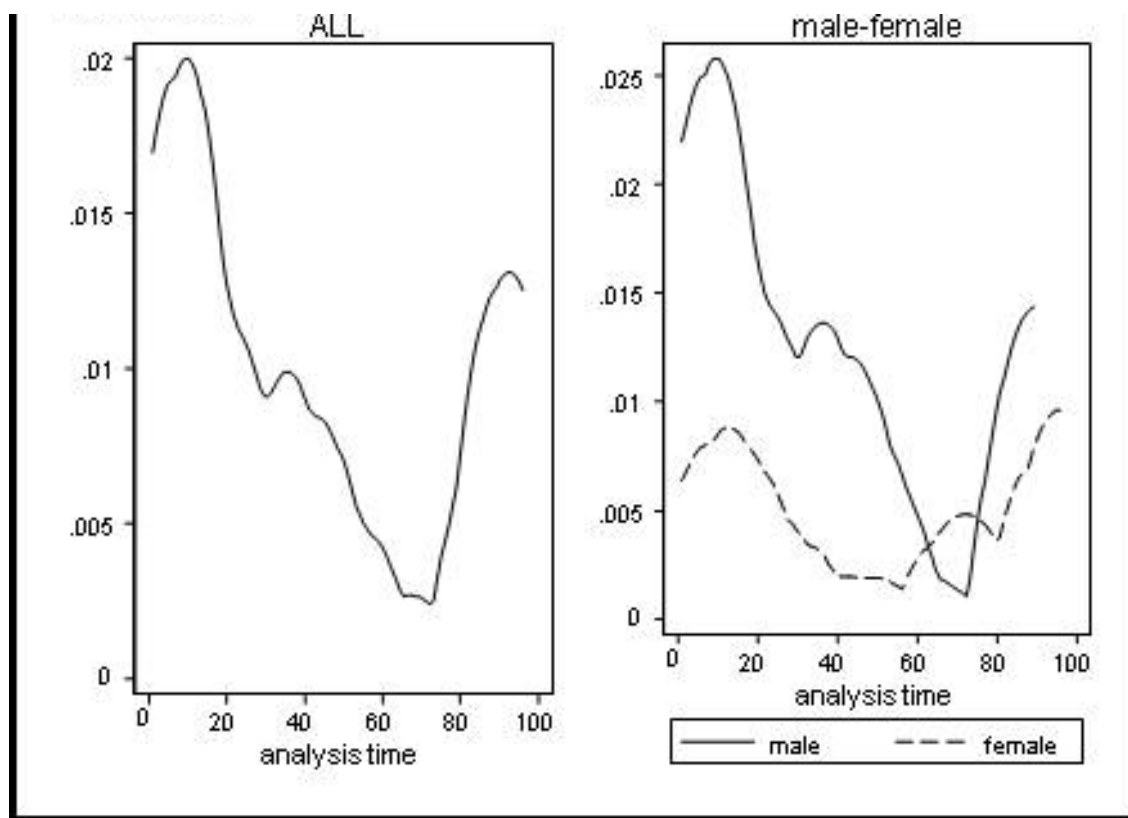
Figure 3: Smoothed Hazard Function under ILO Definition
