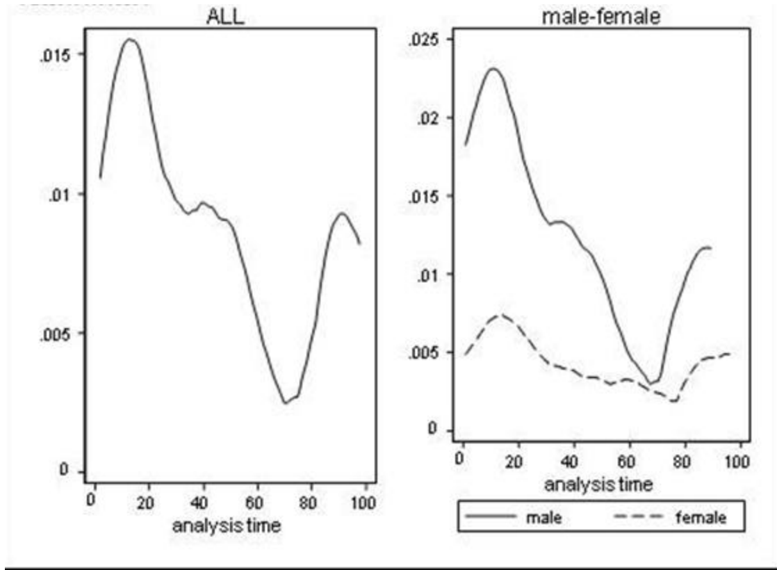
Figure 4: Smoothed Hazard Function under Broad Definition
