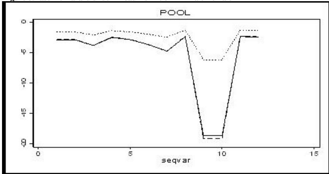
Figure 6: Baseline Hazard under Broad Definition All-Male-Female
