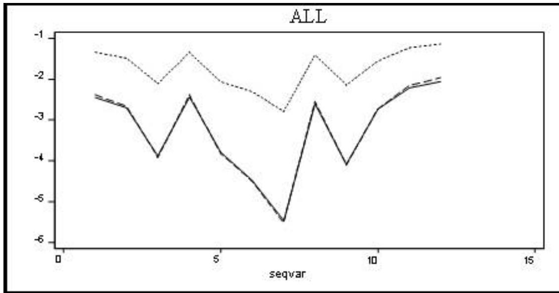
Figure 5: Baseline Hazard under ILO Definition: All Data-Male-Female
