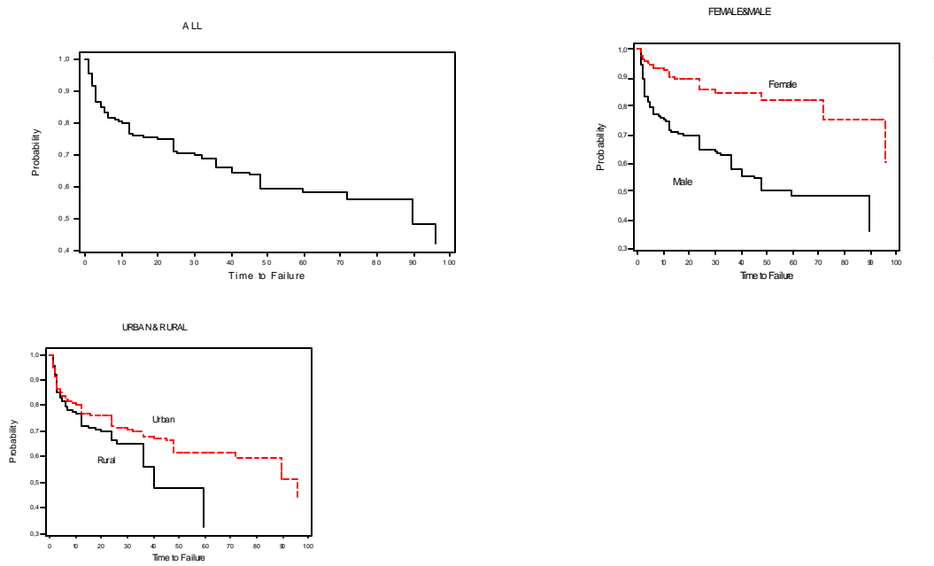
Figure 1: Turnbull's Survival Function under ILO-Definiton
