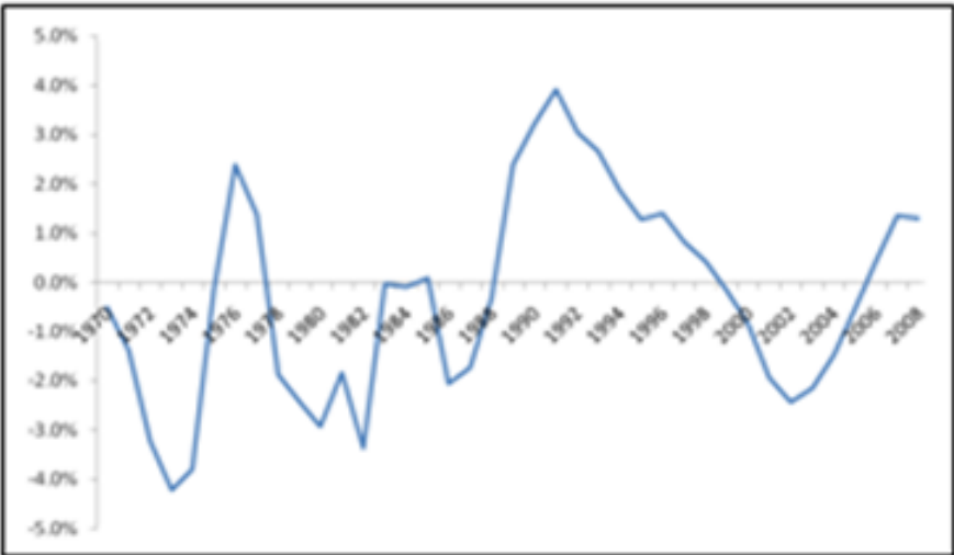
Figure 9: TFP Growth 1970 –
