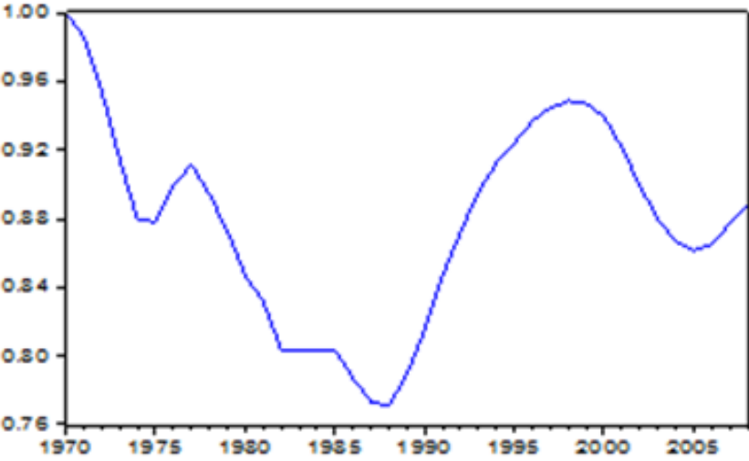
Figure 10: TFP Levels 1970-2008
