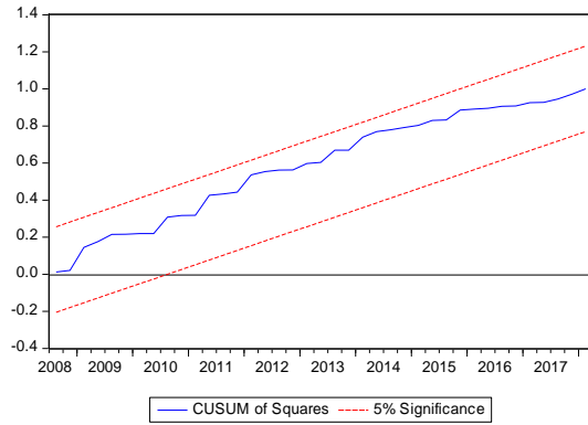
Model 1 INF_UNC
