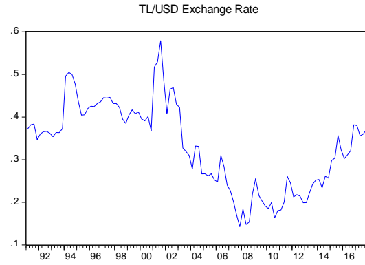
Model 2 INF_UNC
